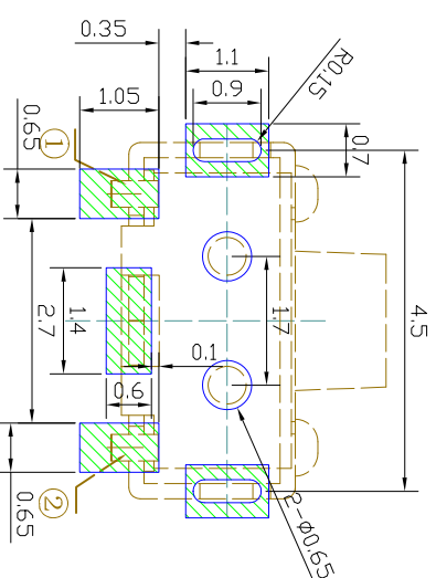
P.C.B MOUNTING PATTERN DIMENSION the following soldering are recommended for reflow soldering
